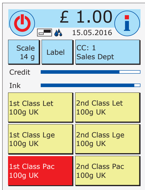
Matrix F82: Original size image
